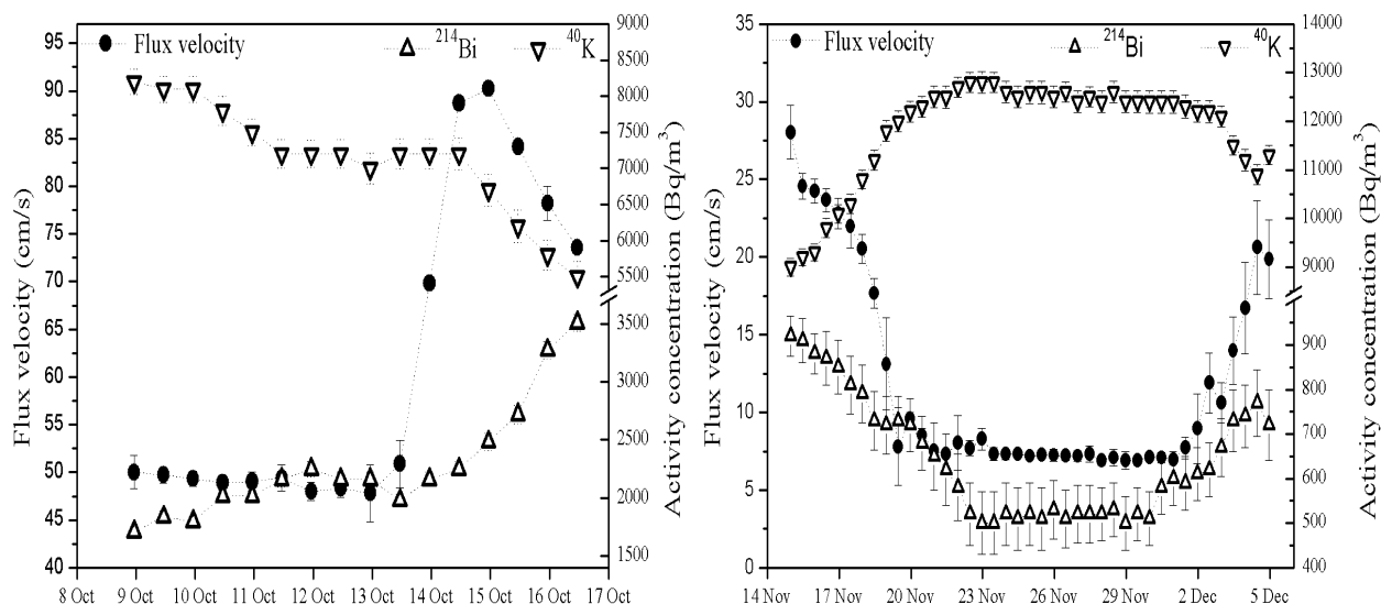
Figure 2: The activity concentration of radon progeny ^{214}\text{Bi} and potassium ^{40}\text{K} as time-series in respect with the velocity of the emanating groundwater. The radon progeny of ^{214}\text{Pb} was found in radioactive equilibrium with ^{214}\text{Bi}
