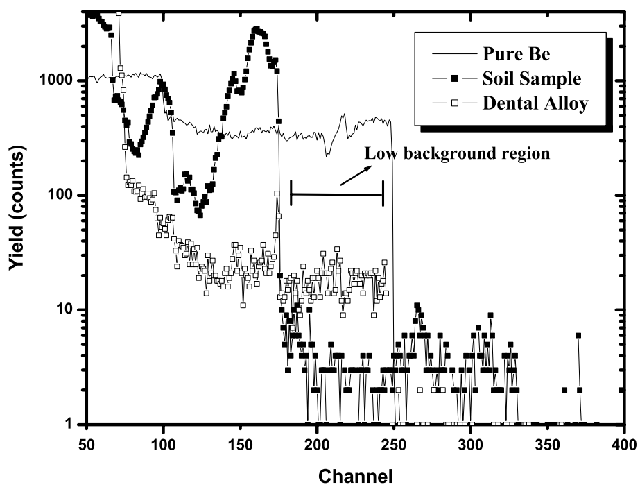
Figure 1: Spectra from the (d,a) and (d,p) reactions at 1.5 MeV deuteron beam for 4\mu\text{Cb} accumulated charge. a) Metallic Be target, b) dental alloy c) Typical soil sample.
