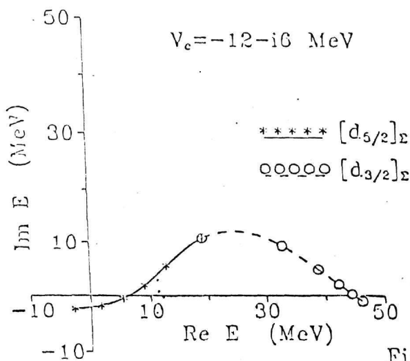
Fig. 4. The position of the poles in the E -plane, when the central potential parameter is V_c = -12 - i6 MeV and the spin-orbit parameter varies, V_{so} = 0, 10, \dots, 50 MeV. The common point of the [d_{5/2}]_\Sigma (solid) curve and of the [d_{3/2}]_\Sigma (dashed) curve corresponds to V_{so} = 0 MeV.
