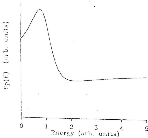
Fig. 3. The resonant part of the production strength S_1(E) , as function of E .
