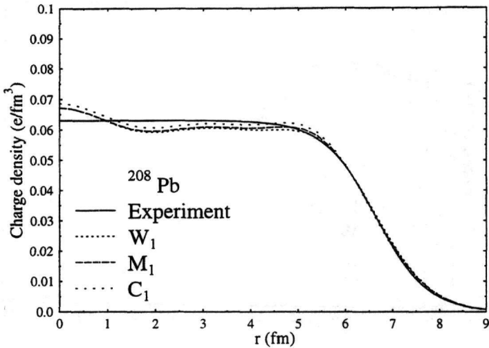
Fig. 3. As for Fig. 1, but for ^{208}\text{Pb}
