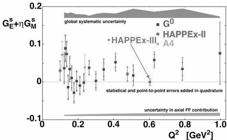
Fig. 6. The combination \mathbf{G}_E^s + \eta \mathbf{G}_M^s for the HAPPEX, A4 and G0 experiments. Also shown at Q^2 = 0.6 \text{ GeV}^2 the projected uncertainty for a future HAPPEX-III measurement.
