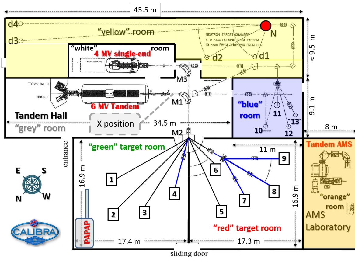
Figure 2: Layout of the electrostatic accelerators as proposed in the full-scale CALIBRA RI. The colored areas indicate building expansions of the current Tandem accelerator lab (in white). The “yellow” room is built under the earth’s surface. The red solid circle labeled “N” is the position of the target for the production of secondary neutrons. In this arrangement, a total number of 13 different beamlines will be available to host dedicated experimental setups. In addition, depending on the desired neutron energy, setups can be installed at different angles with respect to the beam direction, as indicated by the tentative positions marked as d1, d2, d3, and d4.
