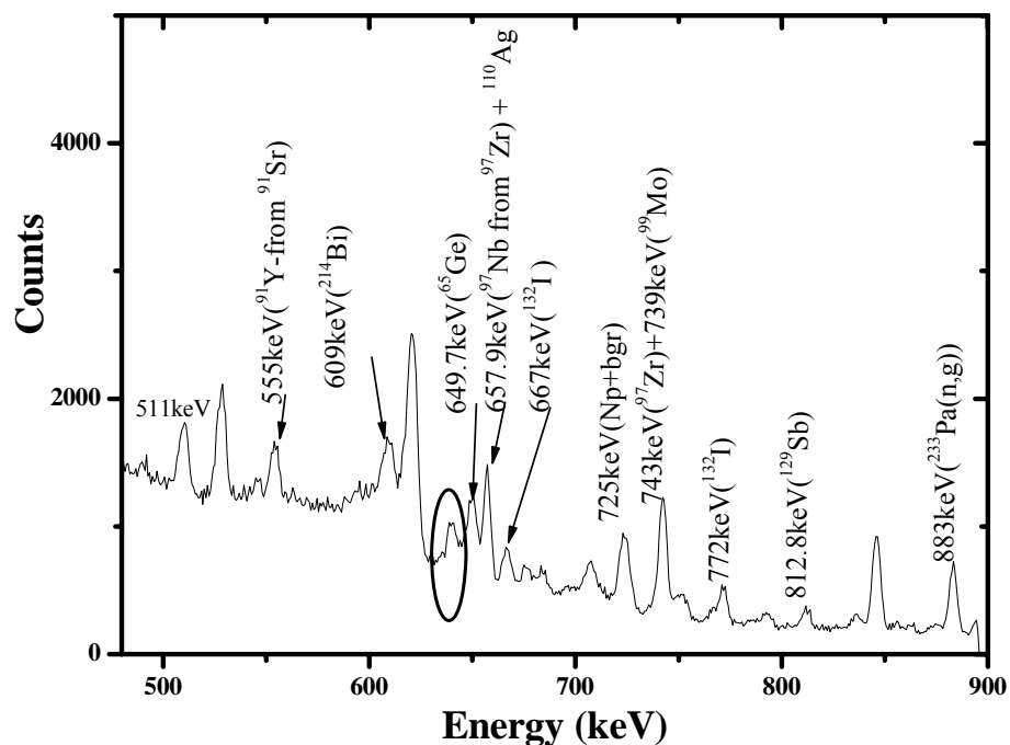
Fig. 5: Calibrated spectrum of the sample after the irradiation ( t_{\text{measurement}}=10\text{h} ), zoomed in the energy region of interest. The gamma ray energy of interest 642 keV is circled at the spectrum.
