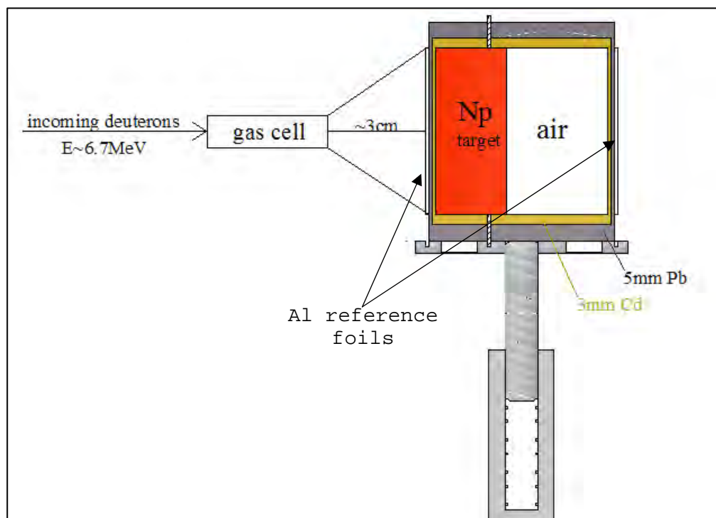
Fig. 3: The setup for the neutron irradiation of the Np target.
