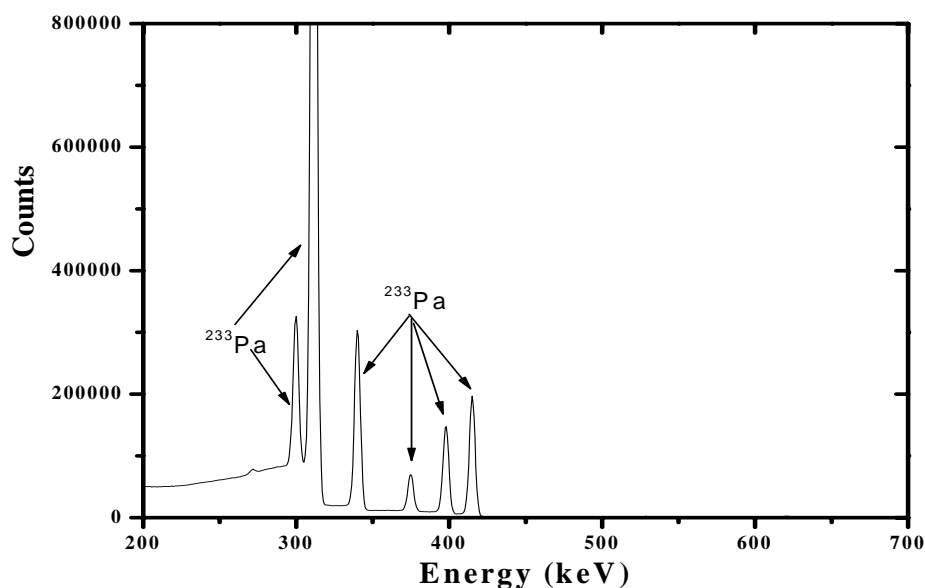
Fig. 4: Calibrated spectrum of the sample before the irradiation.
