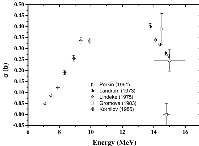
Fig. 1: Existing cross section data for the ^{237}\text{Np}(n,2n) reaction (for the production of the short lived isomer) [8].
