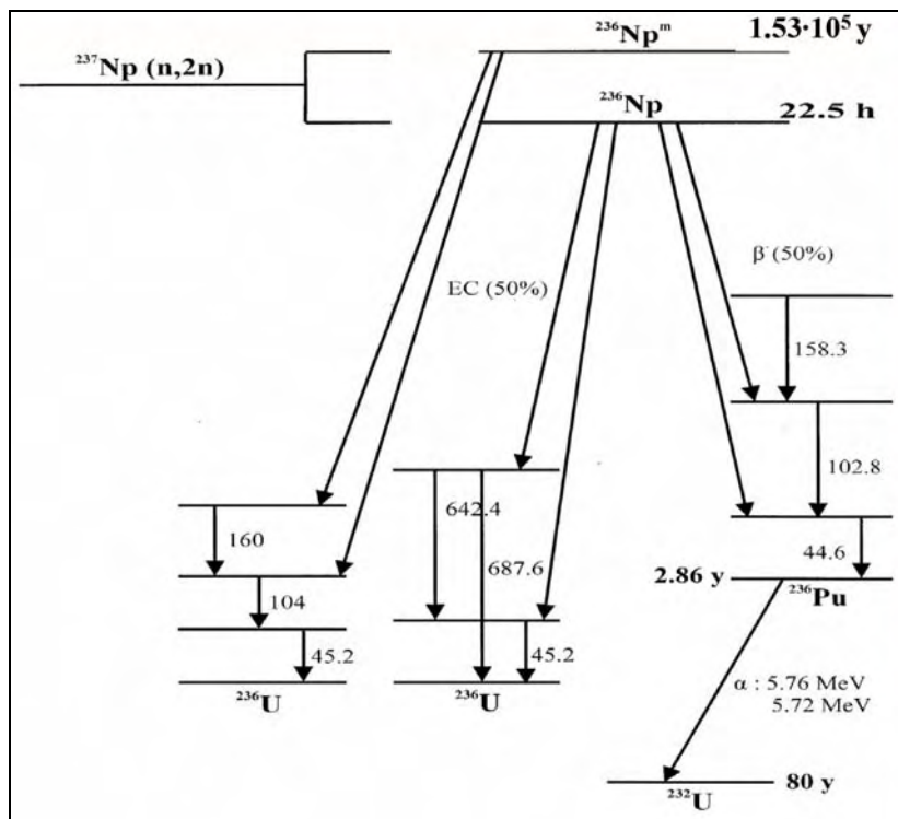
Fig. 2: Decay scheme of the reaction ^{237}\text{Np}(n,2n) . For the long lived isomer of ^{236}\text{Np} only the decay to ^{236}\text{U} (the most probable) has been included in the scheme.
