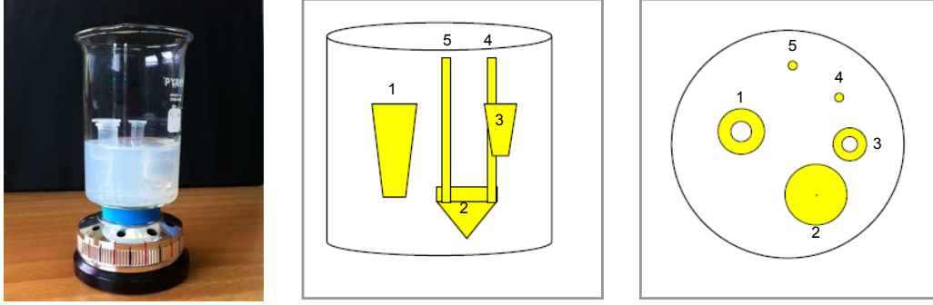
Fig. 2. Picture of the gel-phantom used in the SPECT imaging procedure on its rotating support. The shape and the relative position of the tubes and capillaries is shown in the schematics; they are filled with ^{99m}\text{Tc} water solution (exact volumes and activity are summarized in Table 1) and placed inside the gel.
