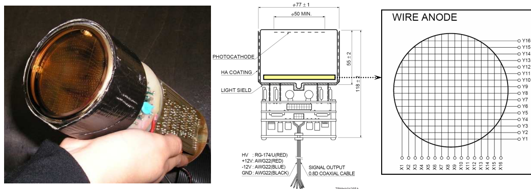
Fig. 1. The small field \gamma -Camera System with the Position Sensitive Photo-Multiplier Tube (PSPMT) and a schematic diagram of its multi-wire anode grid.
