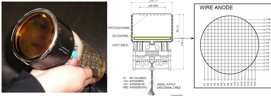
Fig. 1. The small field \gamma -Camera System with the Position Sensitive Photo-Multiplier Tube (PSMPT) and a schematic diagram of its multi-wire anode grid.
