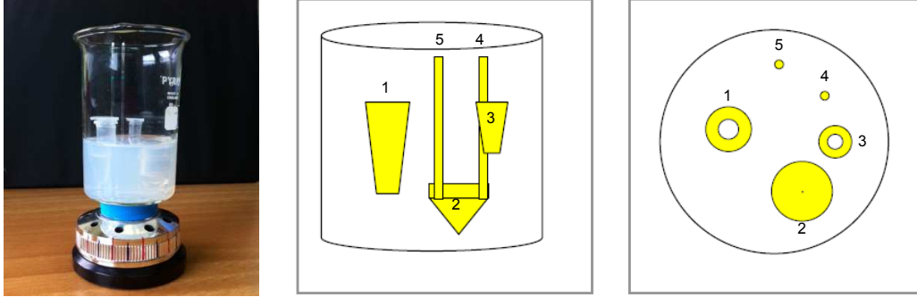
Fig. 2. Picture of the gel-phantom used in the SPECT imaging procedure on its rotating support. The shape and the relative position of the tubes and capillaries is shown in the schematics; they are filled with ^{99m}\text{Tc} water solution (exact volumes and activity are summarized in Table 1) and placed inside the gel.
