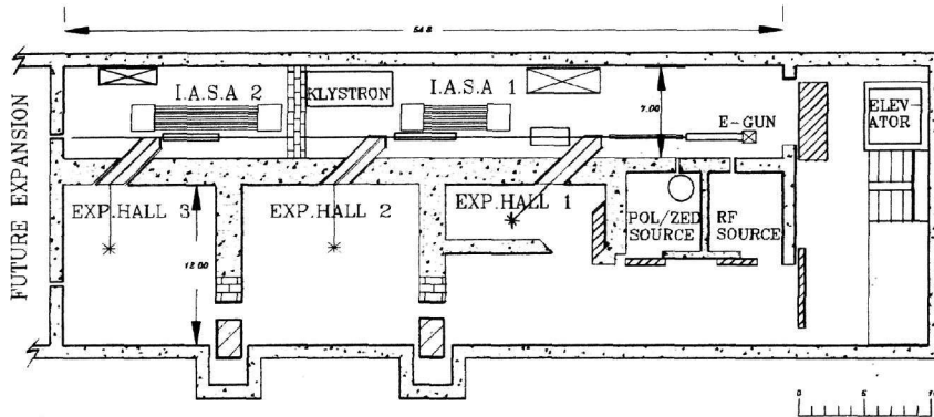
Fig.1 Layout of the IASA RTM facility
