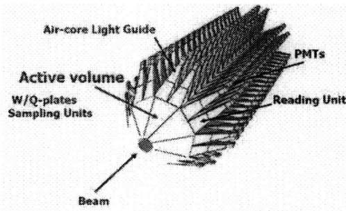
Fig. 1. The CASTOR calorimeter
