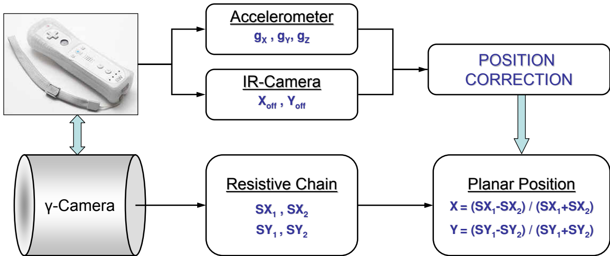
Figure 2: Flow diagram of DAQ recorded parameters during operation of the portable \gamma -Camera System.
