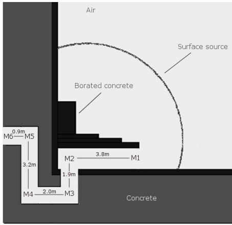
Fig. 1 Cross sectional view of the SW entrance labyrinth
