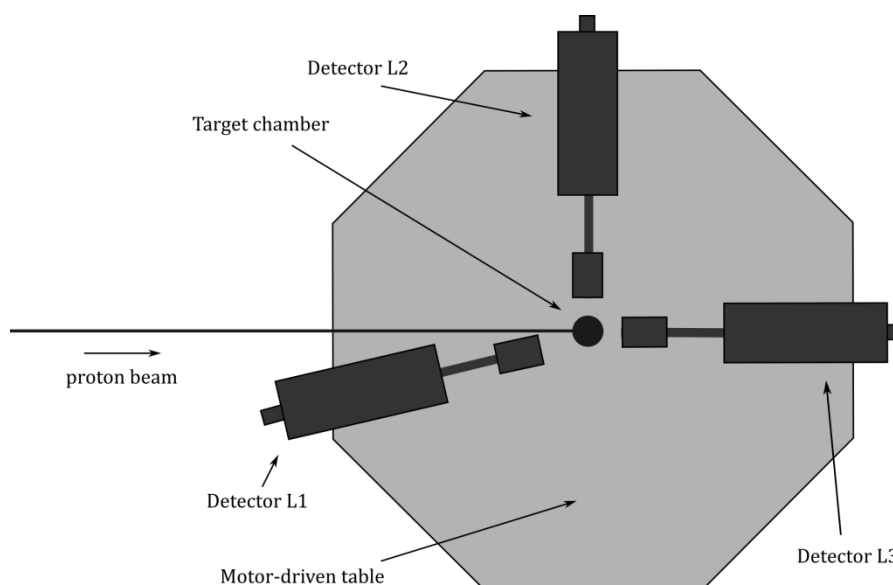
Fig. 1: The detecting setup. Three HPGe detectors are placed in the angles of 0^\circ , 90^\circ and 165^\circ
