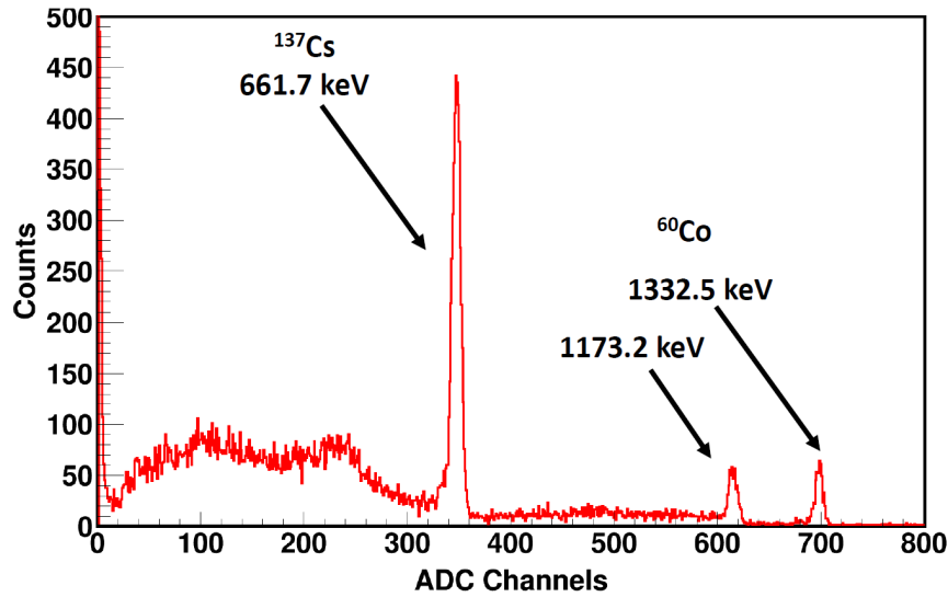
Fig. 2 Amplitude spectra reconstructed from the developed routine in the case of a calibration measurement with ^{137}\text{Cs} and ^{60}\text{Co} radioactive sources. The obtained 1% energy resolution at 661.7 keV, which was in agreement with the resolution of a spectrum recorded with a typical spectroscopy read-out, was satisfactory.
