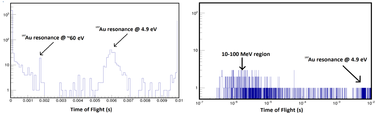
Fig. 3 Reconstructed tof spectra during the irradiation of a ^{197}\text{Au} sample. The 4.9 and 60 eV resonances in the ^{197}\text{Au}(n,\text{tot}) reaction were clearly visible. Promising signals were also reconstructed at neutron energies in the 10-100 MeV region.
