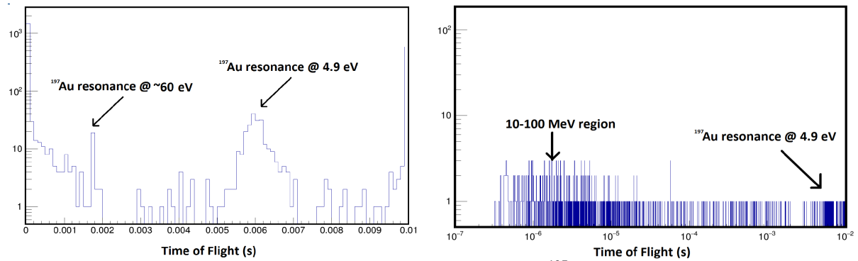
Fig. 3 Reconstructed tof spectra during the irradiation of a ^{197}\text{Au} sample. The 4.9 and 60 eV resonances in the ^{197}\text{Au}(\text{n,tot}) reaction were clearly visible. Promising signals were also reconstructed at neutron energies in the 10-100 MeV region.
